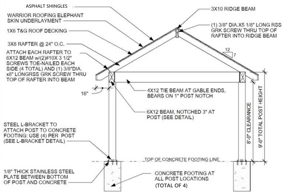
CROSS SECTION
