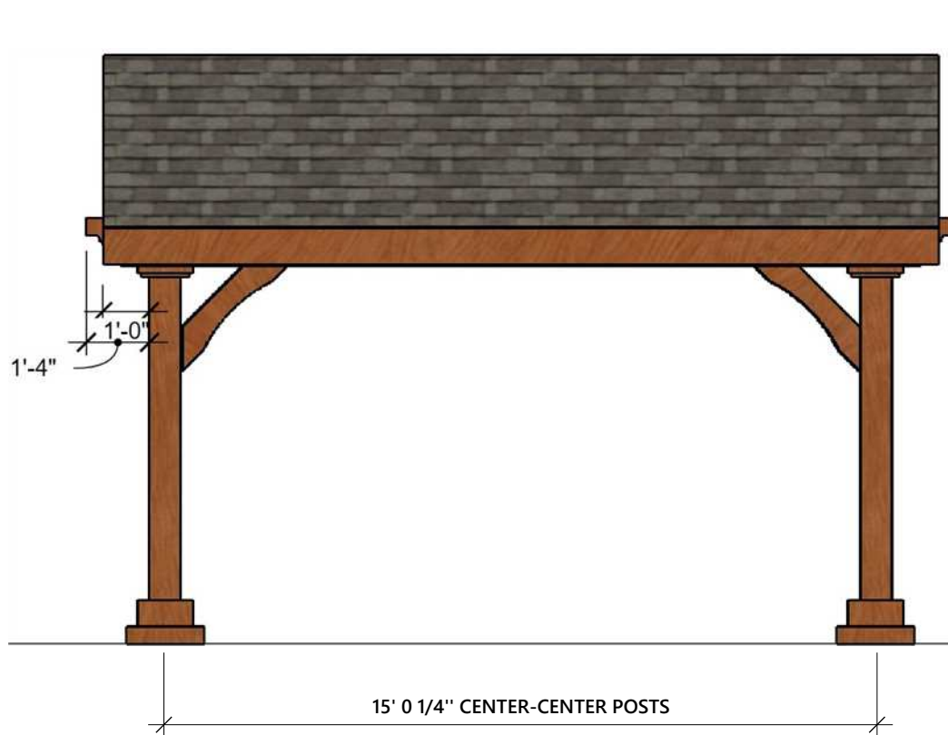
FRONT AND REAR ELEVATION
