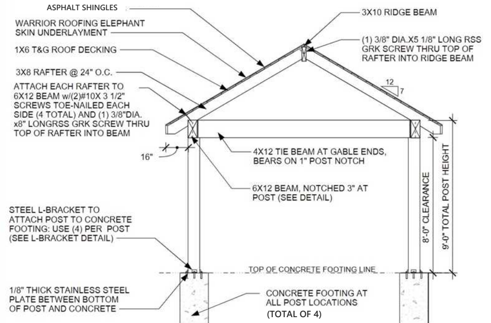
CROSS SECTION
