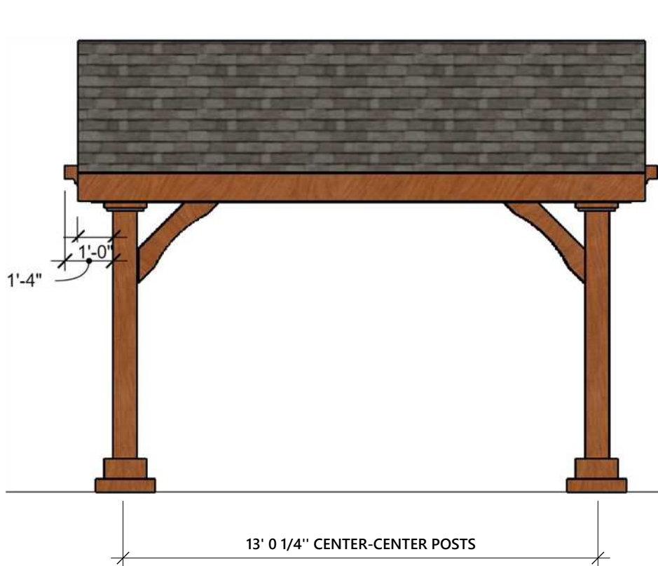
FRONT AND REAR ELEVATION
