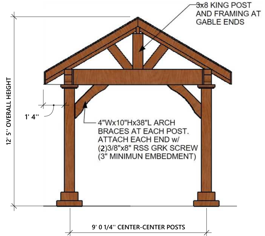
LEFT AND RIGHT ELEVATION
