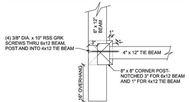
BEAM / POST / TIE BEAM CONNECTION DETAIL
