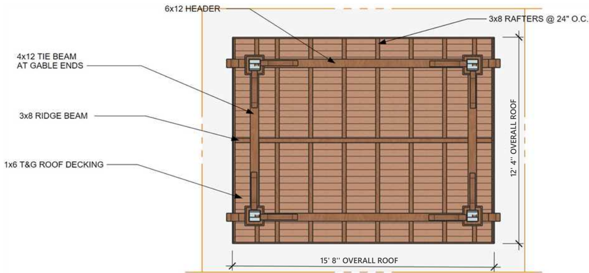
ROOF FRAMING PLAN
