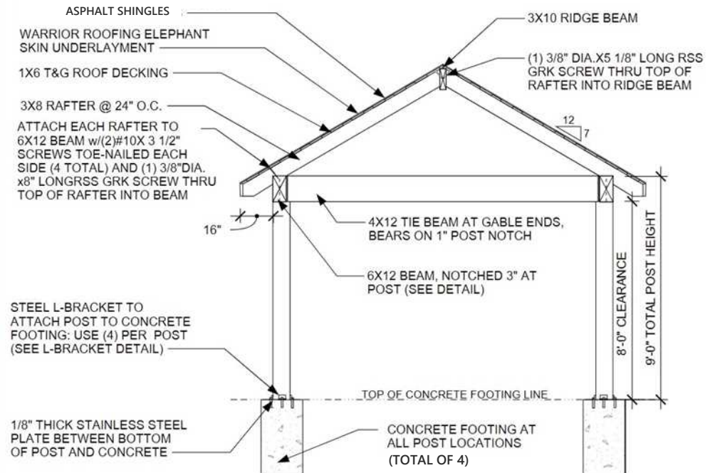
CROSS SECTION
