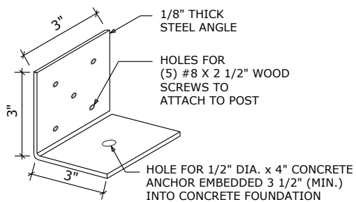
POST L BRACKET DETAIL NO SCALE
