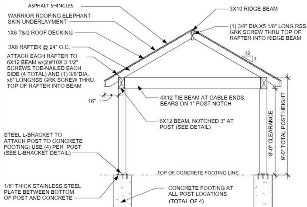
CROSS SECTION
