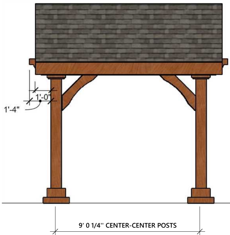
FRONT AND REAR ELEVATION
