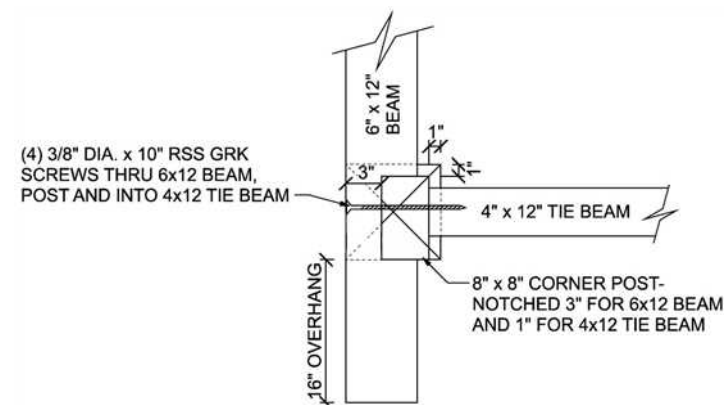
BEAM / POST / TIE BEAM CONNECTION DETAIL
